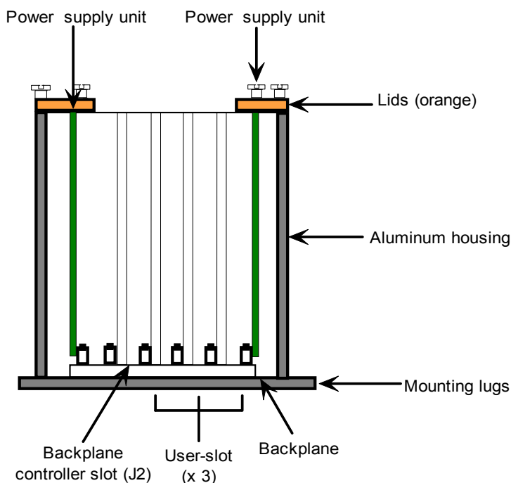
CHS/03U with PSU and three user-slots
